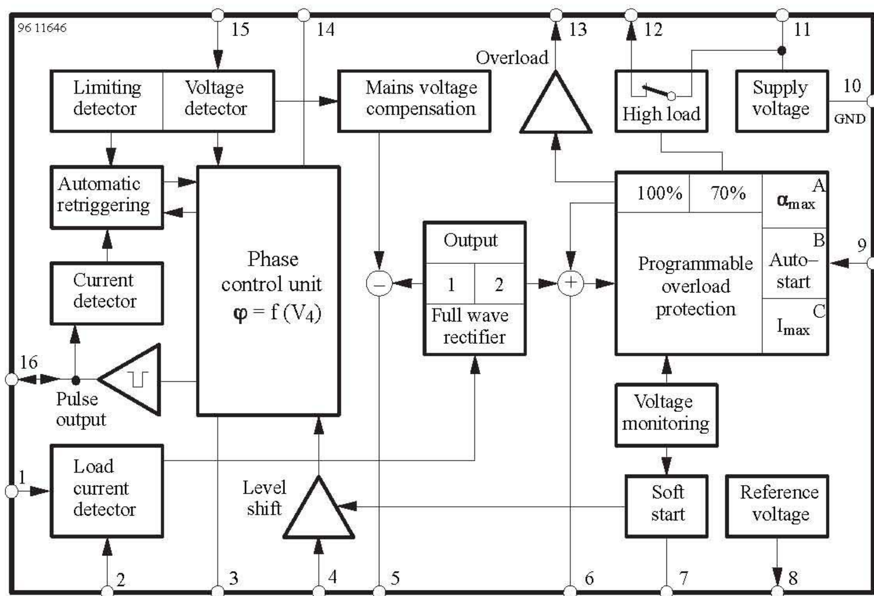
Figure 1. Block diagram
